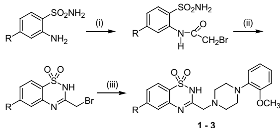
Scheme 1. Reagents and conditions: (i) bromoacetyl bromide, THF anhydrous, room temperature; (ii) 1,4-dioxane, \text{H}_2\text{SO}_4 (few drops), reflux; (iii) 2-methoxyphenylpiperazine, acetonitrile, reflux.
