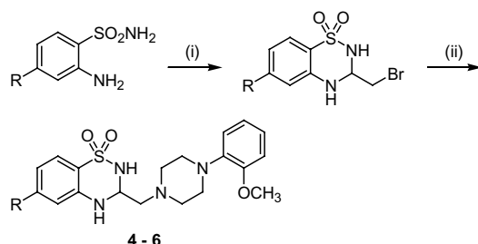
Scheme 2. Reagents and conditions: (i) 2-bromomethyl-1,3-dioxolane, 1,4-dioxane, \text{H}_2\text{SO}_4 (few drops), reflux; (ii) 2-methoxyphenylpiperazine, acetonitrile, reflux.
